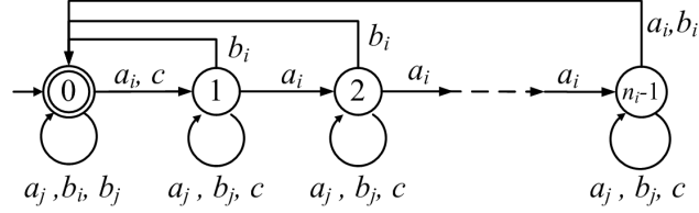
Figure 1: Witness DFA A_i for Theorems 3.2
