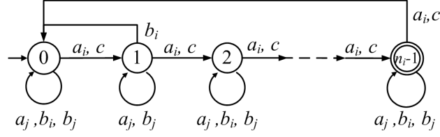
Figure 2: Witness DFA A_i for Theorems 4.2
